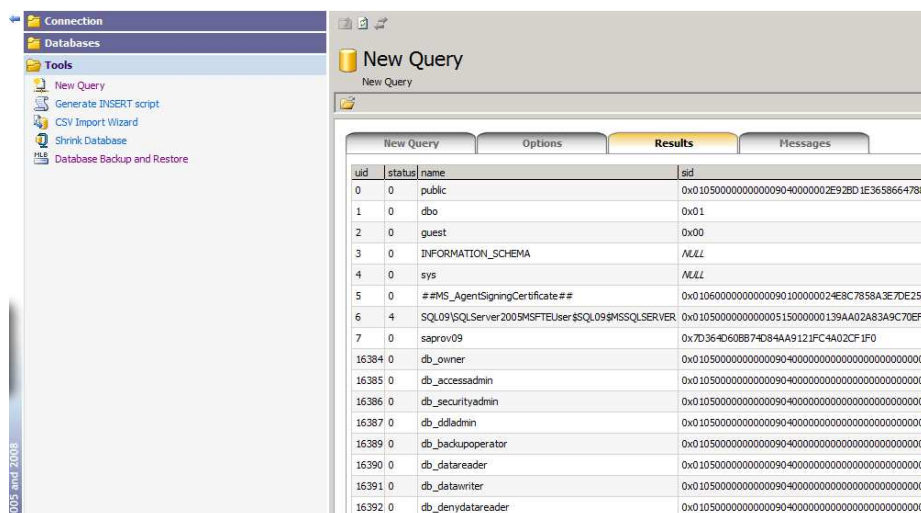
Fig. 11. Querying the master..sysusers table.
