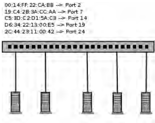
Fig. 2. A switch and its CAM table.
