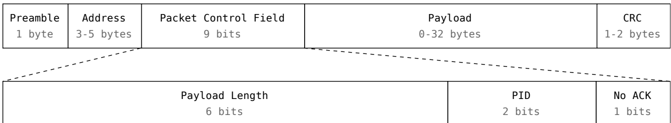
Figure 2: Enhanced Shockburst packet format
